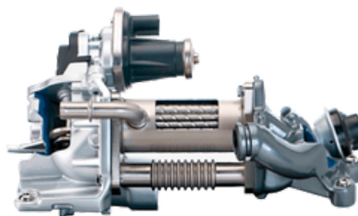
EGR System
