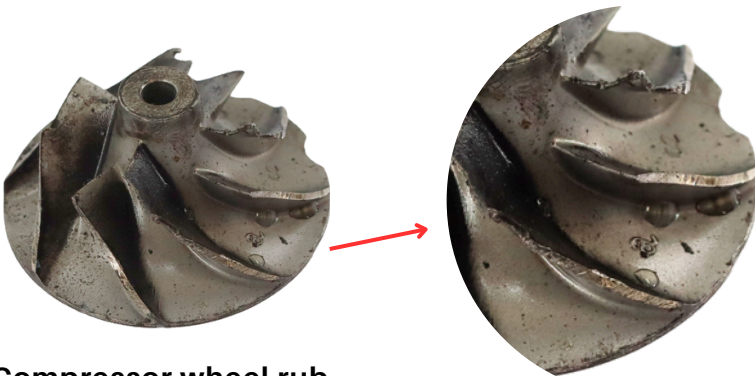
Compressor wheel rub
